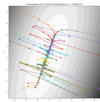
(g) Iterates for various preconditioners.
