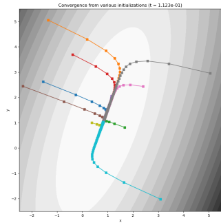
(a) Iterates for various preconditioners.
