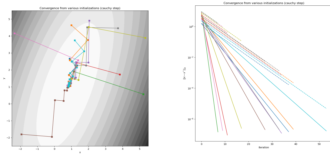
(b) Error \|x^{(k)} - x^*\|_A . Dashed lines indicate the linear convergence bound.
