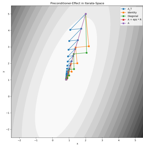
(a) Iterates for various preconditioners.
