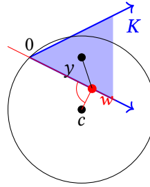
Figure 7.3: Illustration of the construction of the normal vector d = w - c of the separating hyperplane (red) in the proof of the Farkas-Lemmas 7.11.
