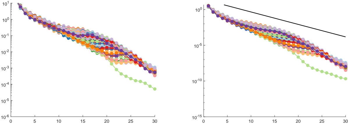
(a) The norm of the gradient \sqrt{\delta^{(k)}} = \|\nabla_M \phi(x^{(k)})\|_M = \|r^{(k)}\|_{M^{-1}} does not necessarily converge monotonically.
